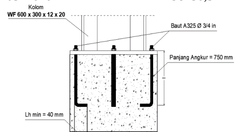
Gambar 8. Penampang Base Plate
