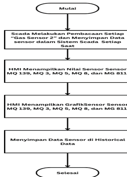
Gambar 24. Flowchart Gas Sensor 2
