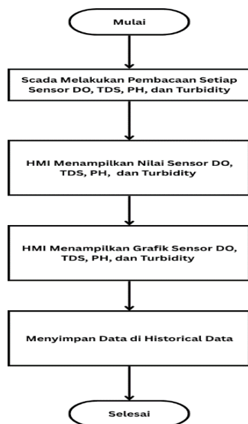
Gambar 22. Flowchart Water Sensor
