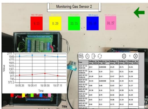
Gambar 47. Tampilan Monitoring Gas Sensor 2
