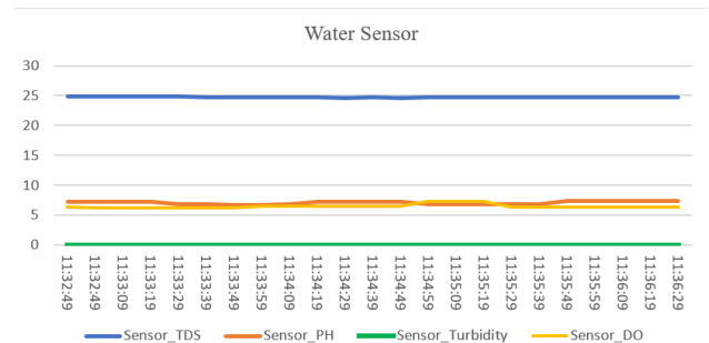
Gambar 35. Grafik Water Sensor
